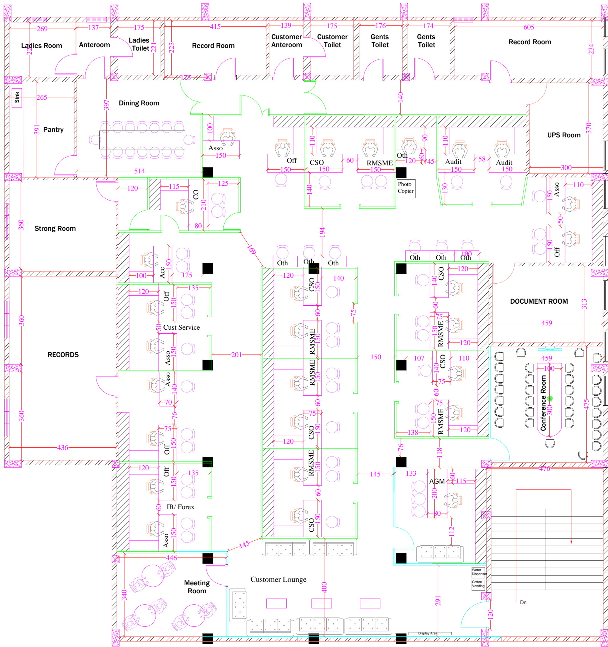
Proposed Interior Layout of SME ERNAKULAM BRANCH- Revision 2A
